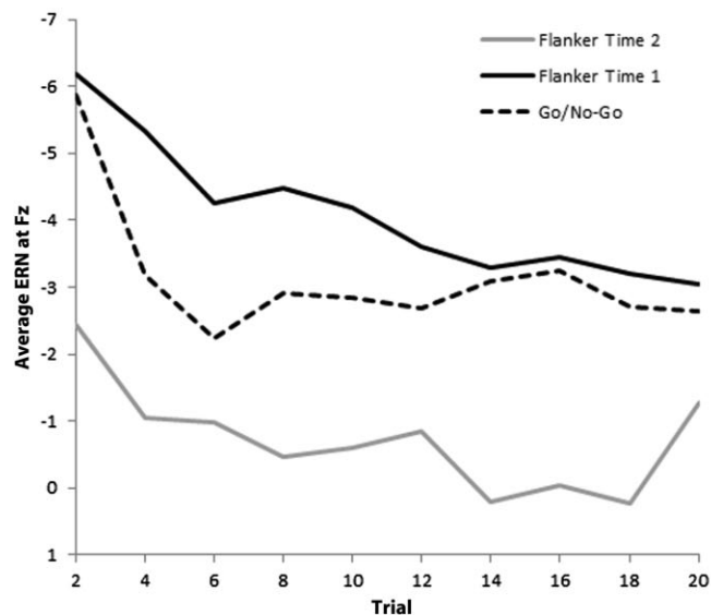
Figure 3. Magnitude of the ERN at Fz (left) and Cz (right) as a function of error number for the flanker task at Time 1 and 2, and the go/no-go task at Time 2.
