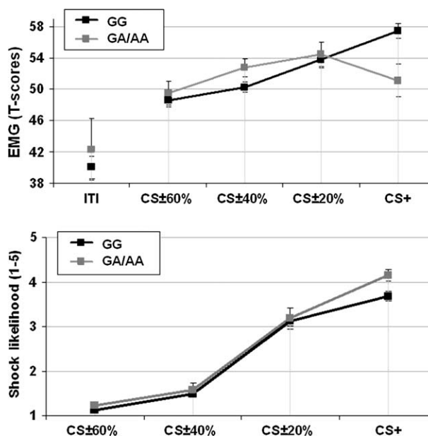
Figure 1: Startle response magnitude and post-task shock likelihood ratings as a function of stimulus type. Standardized EMG activity elicited by startle probes (top) and behavioral ratings of shock likelihood (bottom; 1 = “certainly not shocked”, 5 = “certainly shocked”) for each stimulus type for both individuals carrying the Val/Val BDNF genotype ( N = 44 ) and those carrying one or two Met alleles of the BDNF genotype ( N = 13 ).
